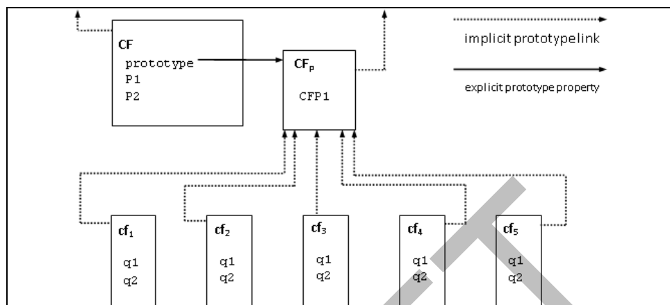
Figure 1 — Object/Prototype Relationships
